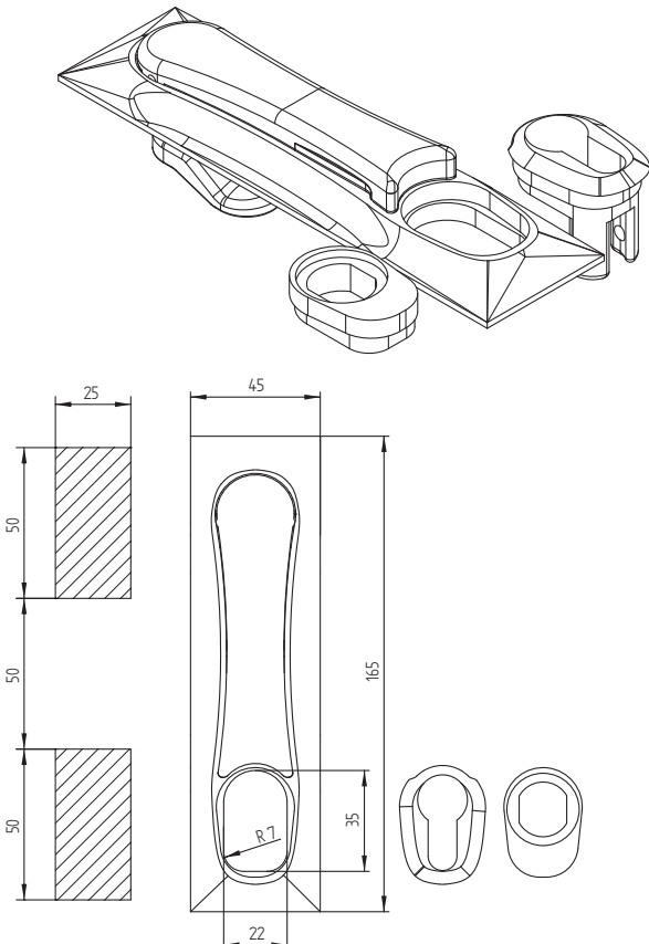
New handle
