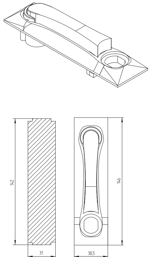
Former handle
